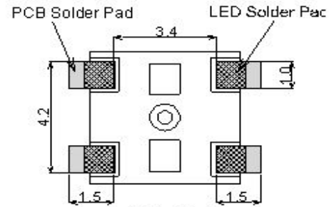
Solder Pad
